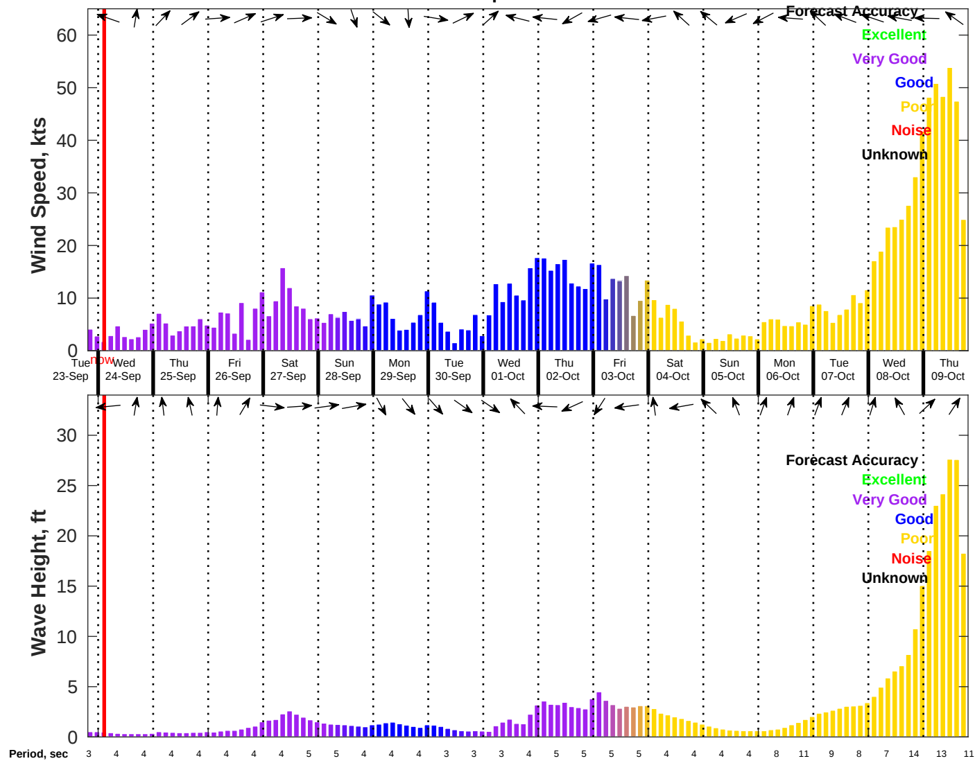
Wind & Wave Forecast for NDBC 42036 from 23-Sep-2025 19:00:00 to 09-Oct-2025 19:00:00
