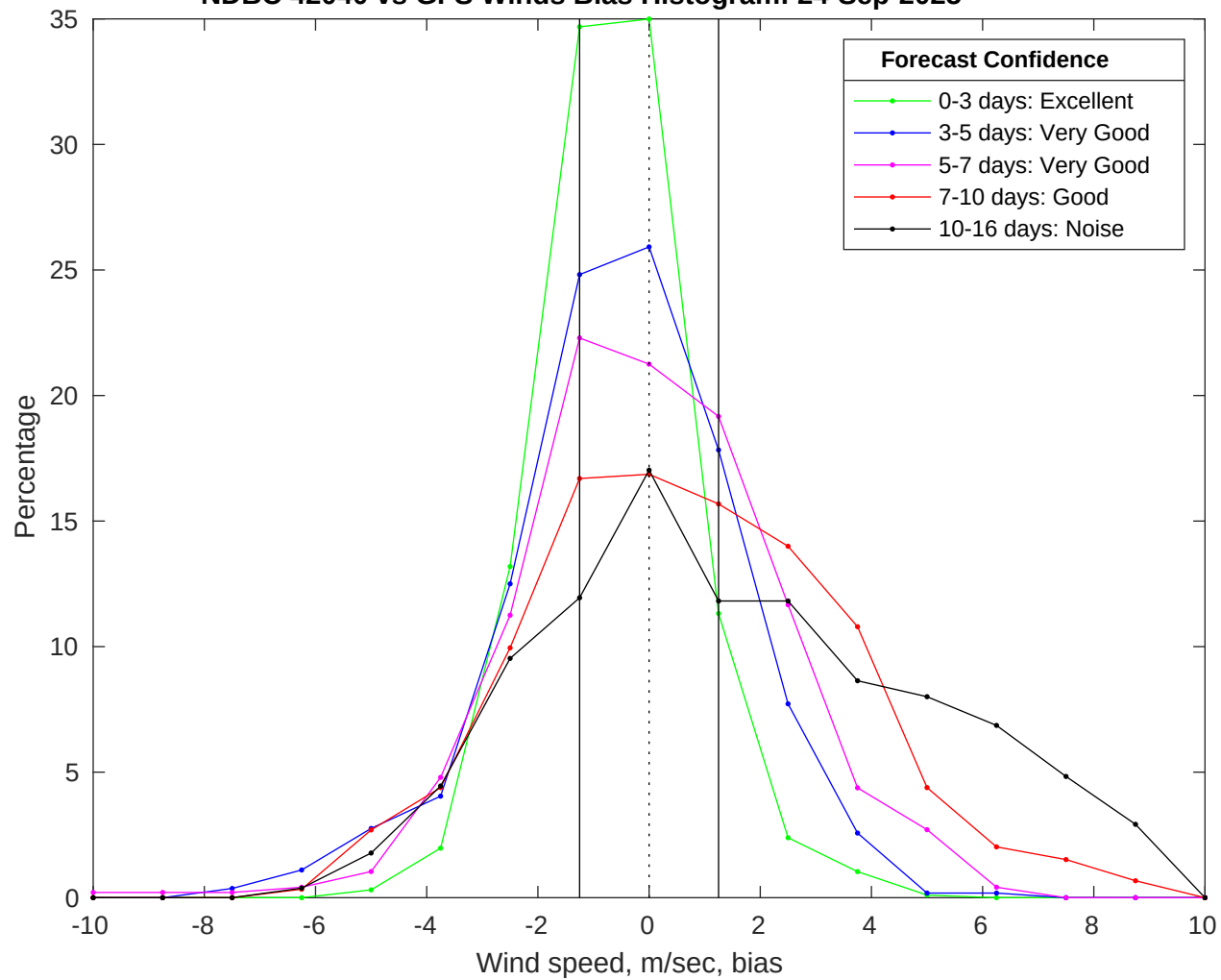
NDBC 42040 vs GFS Winds Bias Histogram: 24-Sep-2025
