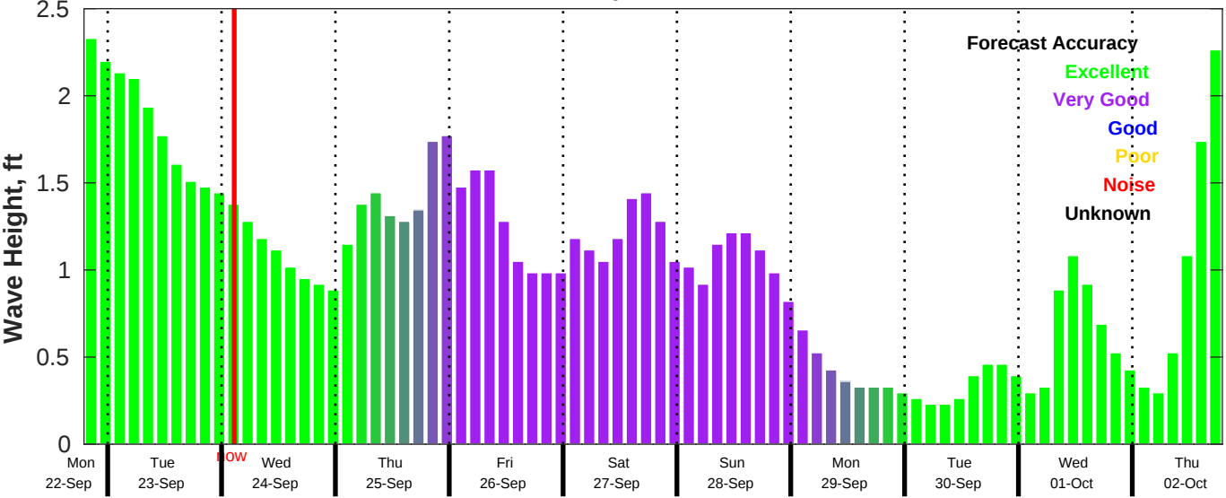
CMEMS Wave Forecast for NDBC 42040 from 22-Sep-2025 19:00:00 to 02-Oct-2025 19:00:00
