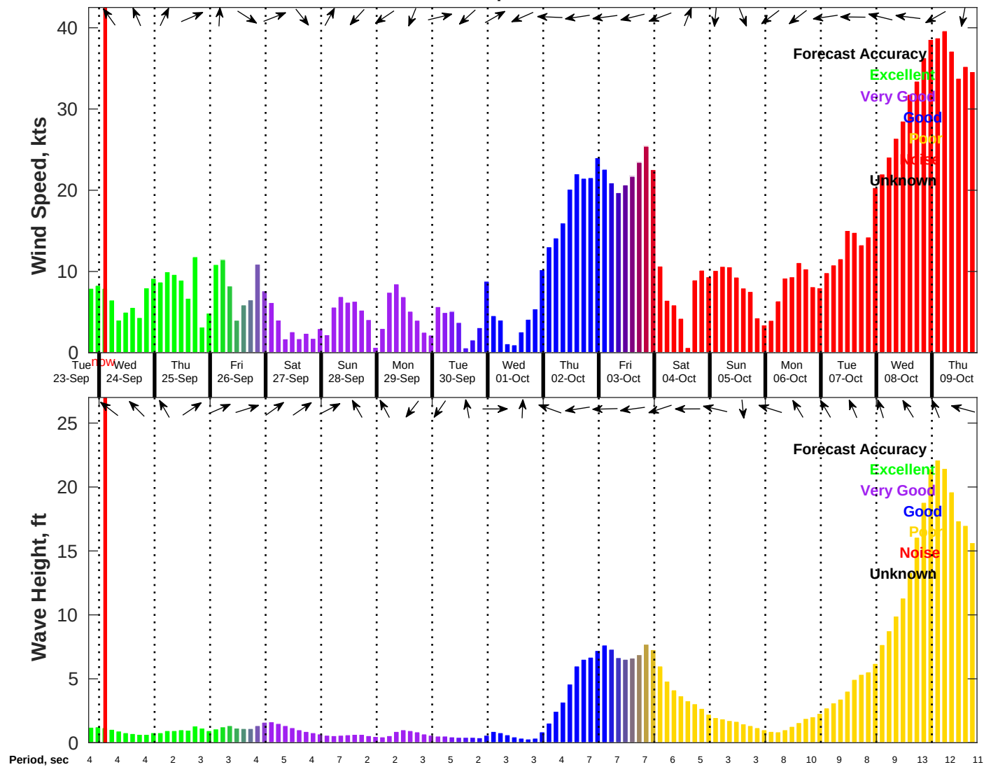
Wind & Wave Forecast for NDBC 42040 from 23-Sep-2025 19:00:00 to 09-Oct-2025 19:00:00
