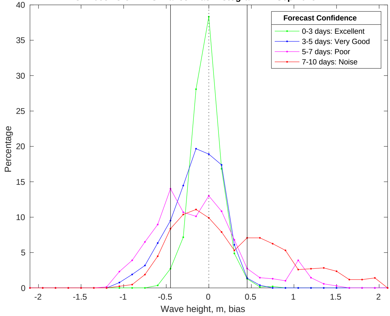
NDBC 44008 vs CMEMS Waves Bias Histogram: 24-Sep-2025
