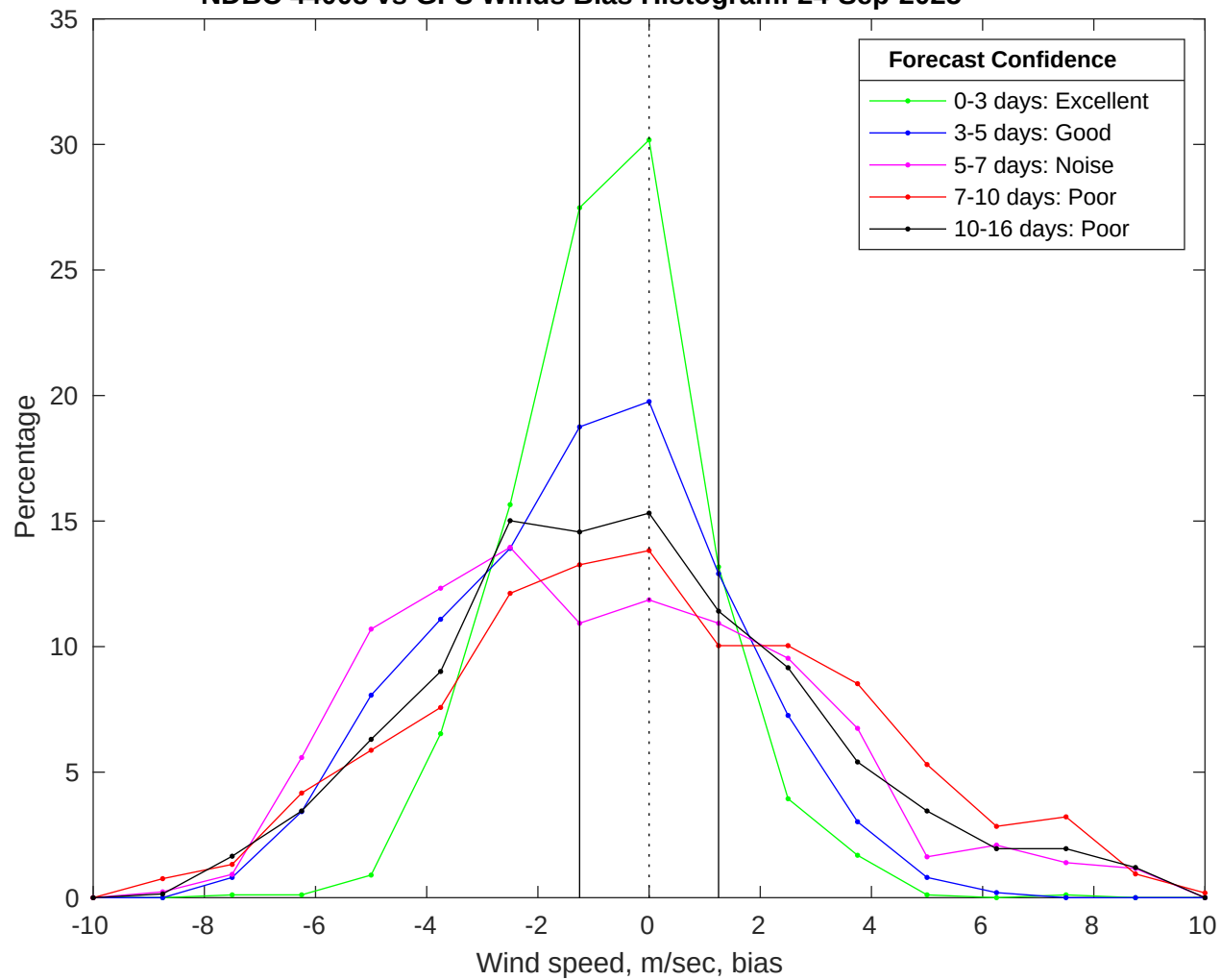
NDBC 44008 vs GFS Winds Bias Histogram: 24-Sep-2025
