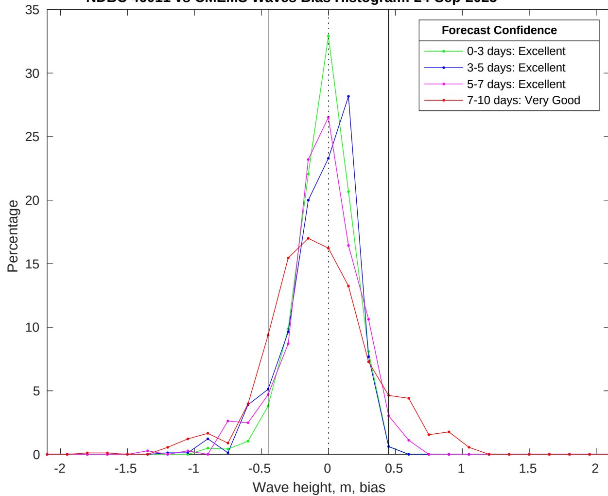
NDBC 46011 vs CMEMS Waves Bias Histogram: 24-Sep-2025
