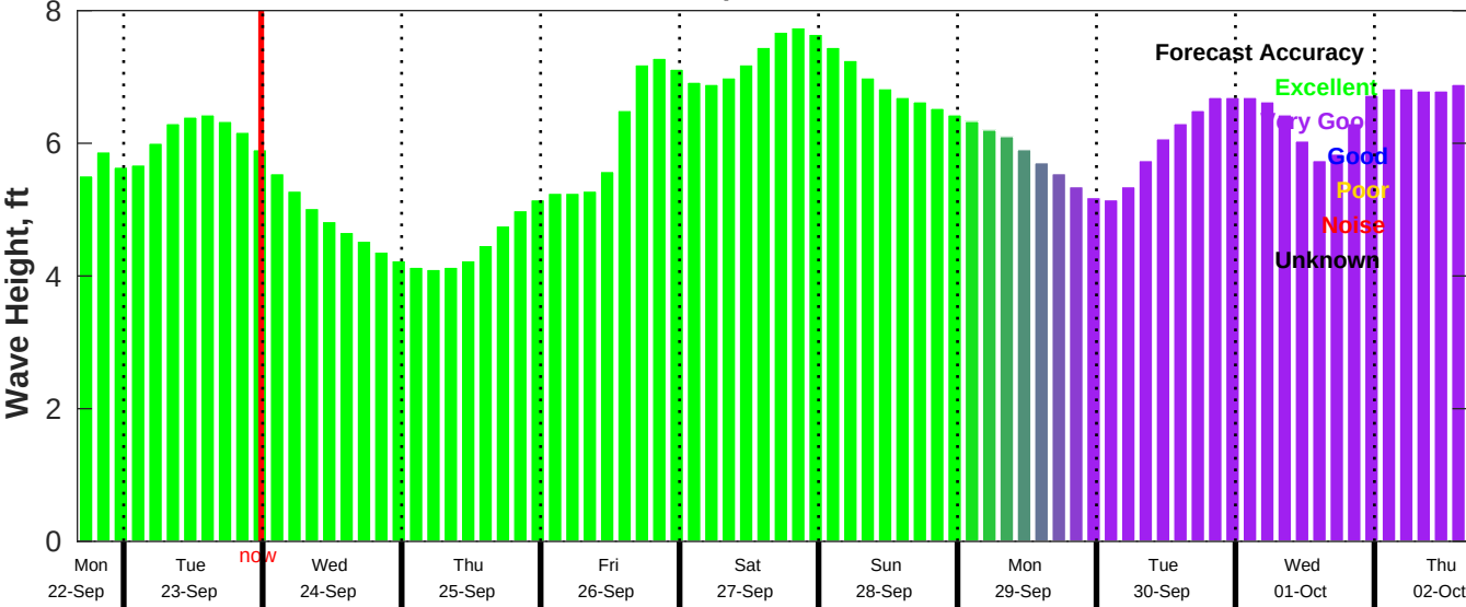
CMEMS Wave Forecast for NDBC 46011 from 22-Sep-2025 16:00:00 to 02-Oct-2025 16:00:00
