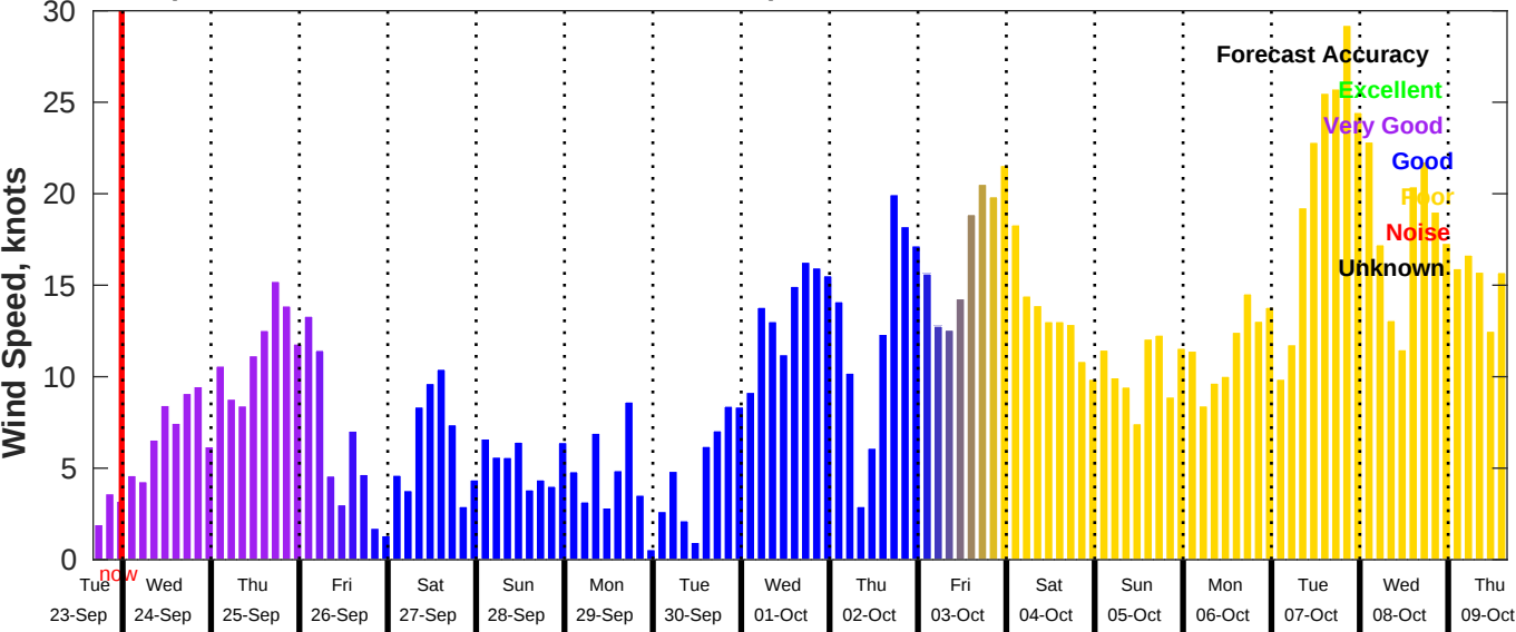
GFS Wind Speed Forecast for NDBC 46011 from 23-Sep-2025 16:00:00 to 09-Oct-2025 16:00:00
