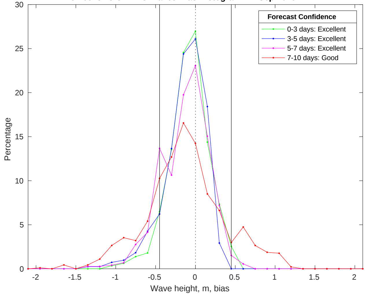
NDBC 46028 vs CMEMS Waves Bias Histogram: 24-Sep-2025
