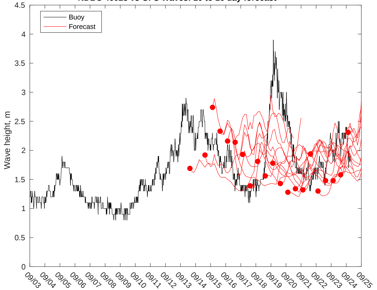
NDBC 46028 vs GFS Waves: 10 to 16 day forecast
