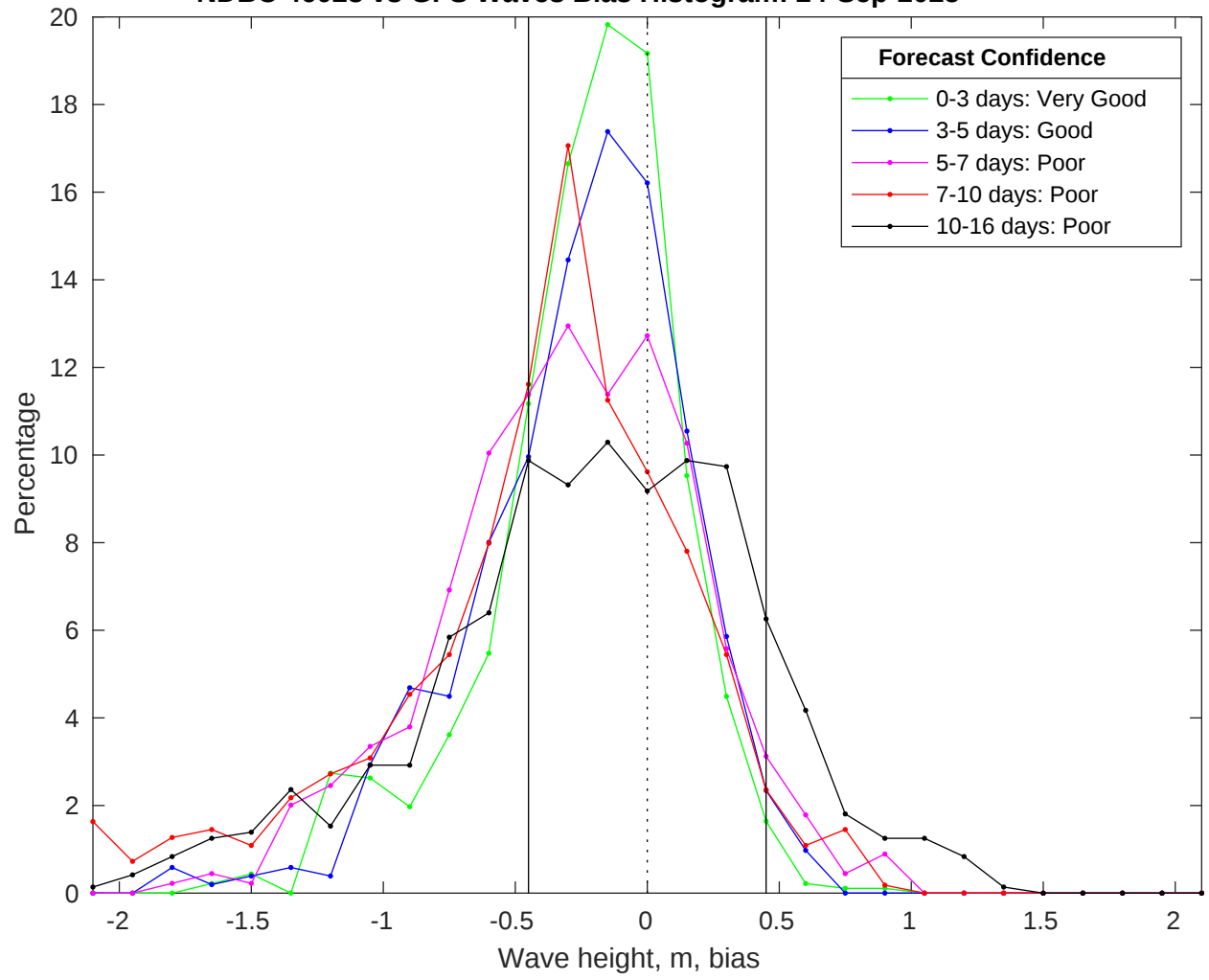
NDBC 46028 vs GFS Waves Bias Histogram: 24-Sep-2025
