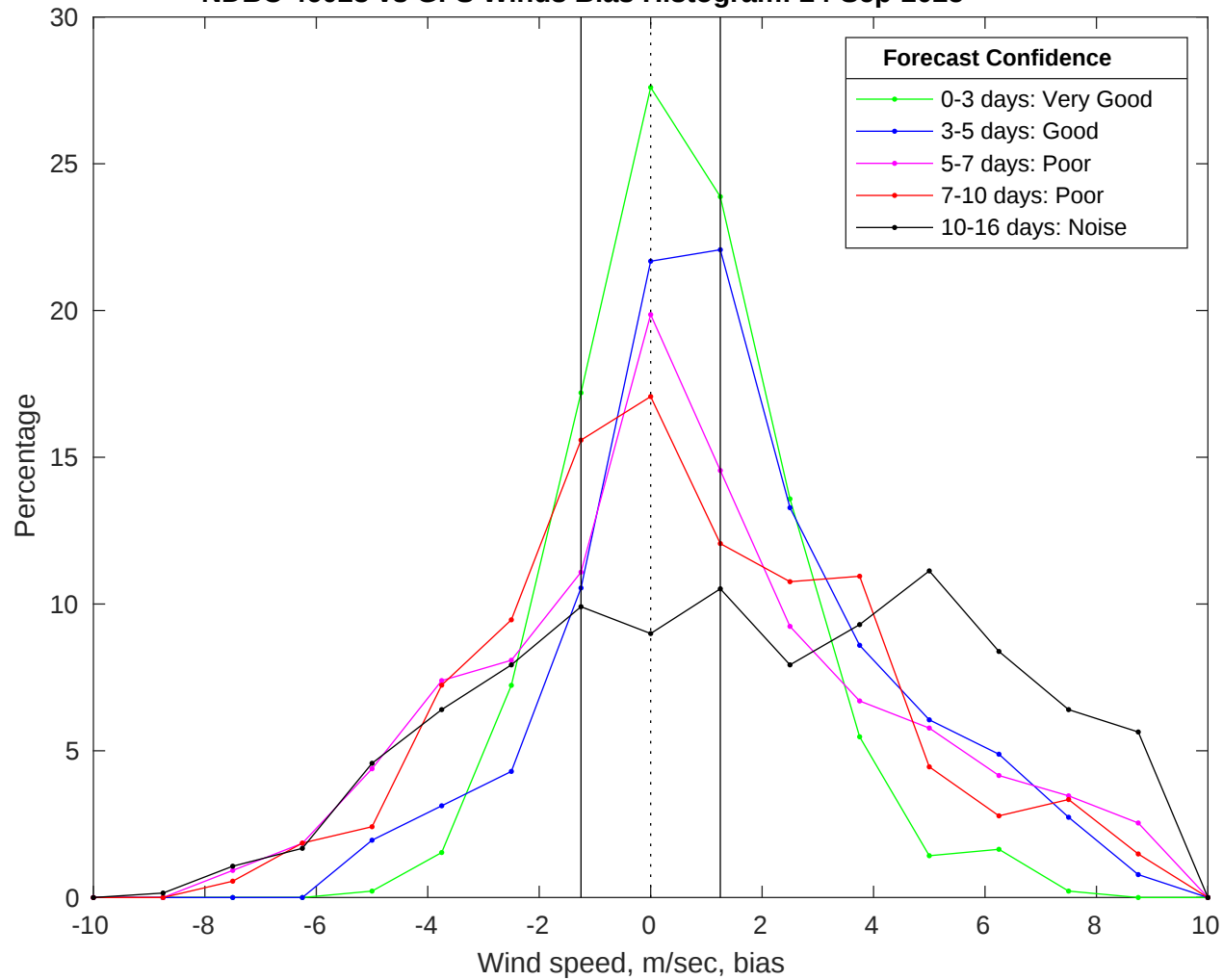
NDBC 46028 vs GFS Winds Bias Histogram: 24-Sep-2025
