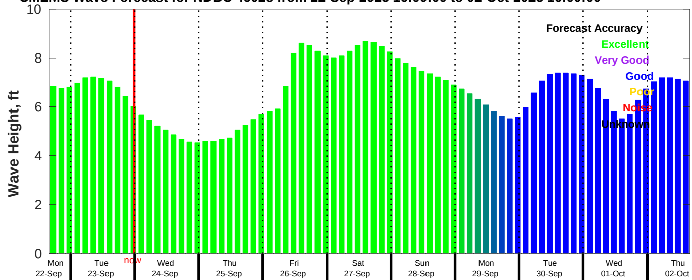
CMEMS Wave Forecast for NDBC 46028 from 22-Sep-2025 16:00:00 to 02-Oct-2025 16:00:00
