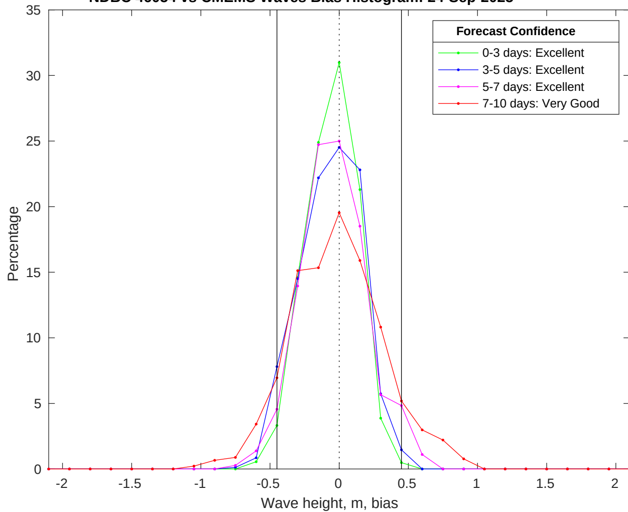
NDBC 46054 vs CMEMS Waves Bias Histogram: 24-Sep-2025
