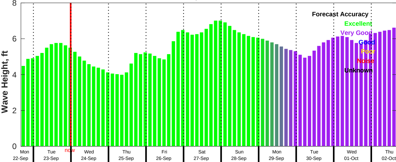
CMEMS Wave Forecast for NDBC 46054 from 22-Sep-2025 16:00:00 to 02-Oct-2025 16:00:00
