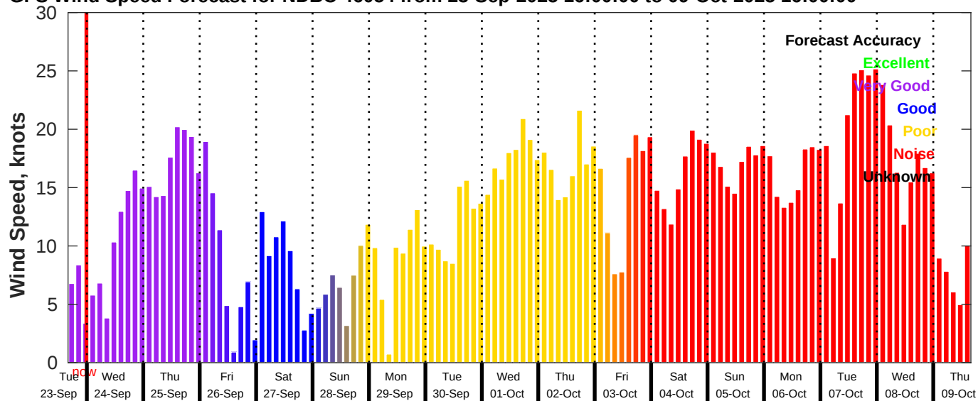
GFS Wind Speed Forecast for NDBC 46054 from 23-Sep-2025 16:00:00 to 09-Oct-2025 16:00:00
