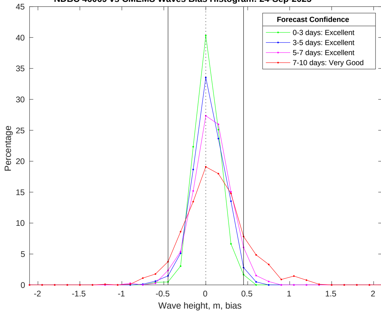
NDBC 46069 vs CMEMS Waves Bias Histogram: 24-Sep-2025
