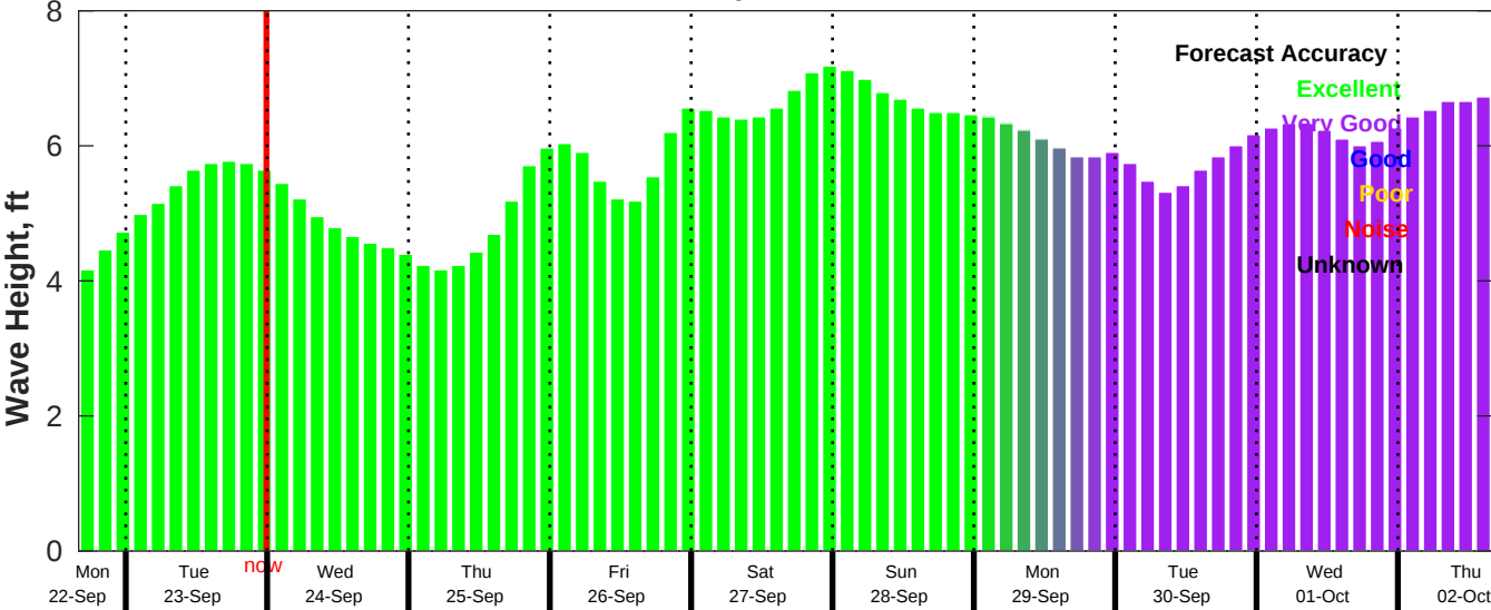
CMEMS Wave Forecast for NDBC 46069 from 22-Sep-2025 16:00:00 to 02-Oct-2025 16:00:00
