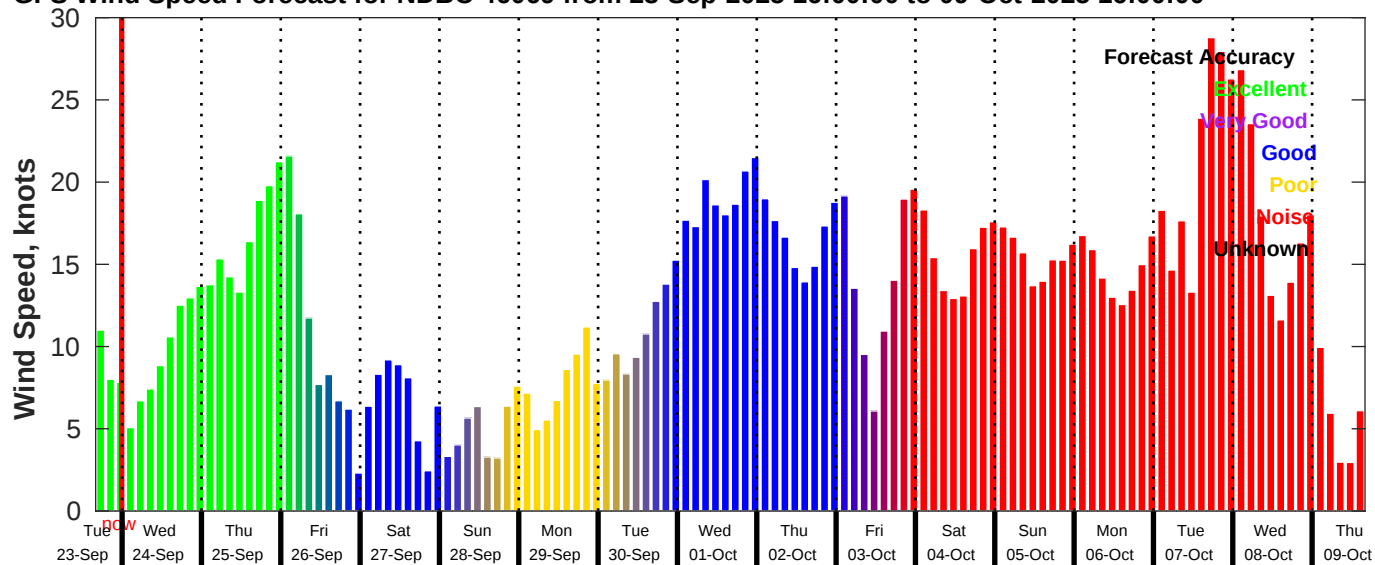
GFS Wind Speed Forecast for NDBC 46069 from 23-Sep-2025 16:00:00 to 09-Oct-2025 16:00:00
