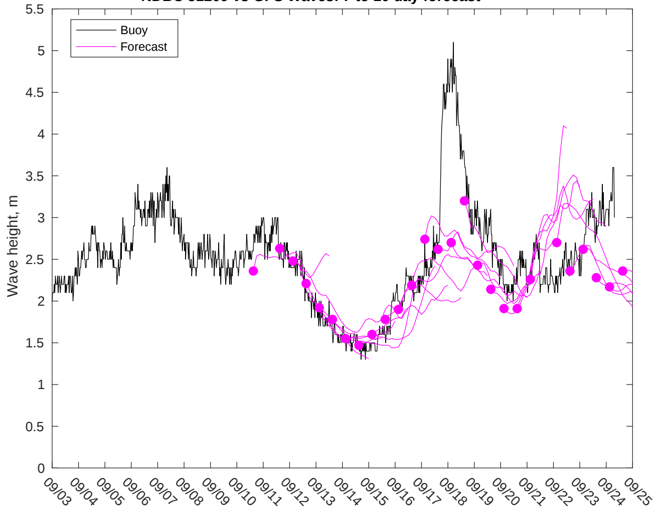
NDBC 51209 vs GFS Waves: 7 to 10 day forecast
