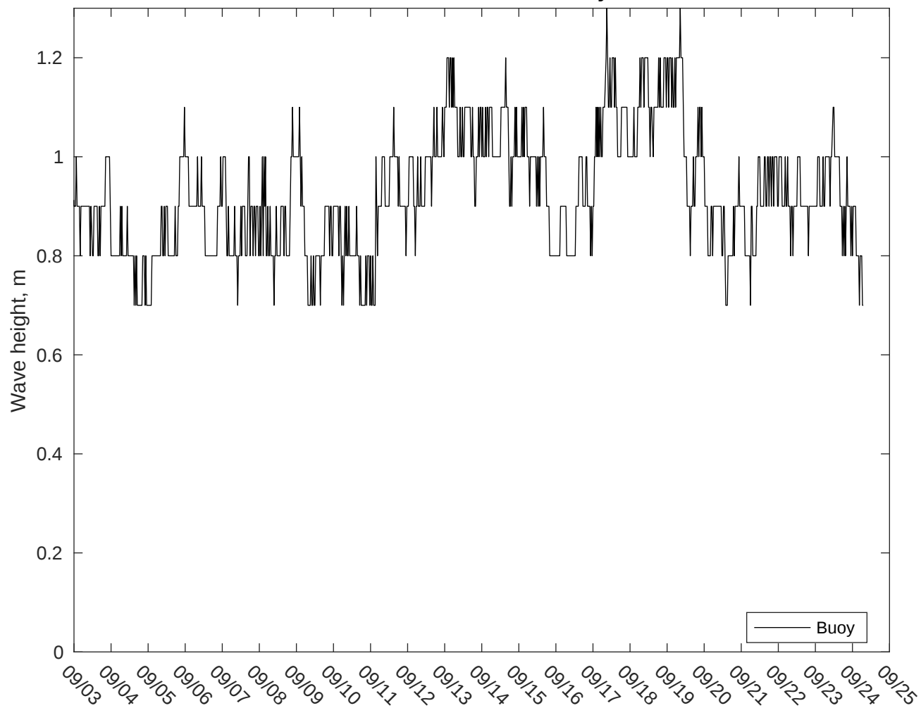
NDBC 51211 vs CMEMS Waves: 10 to 16 day forecast
