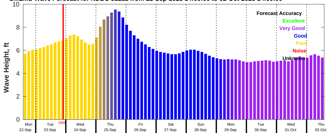
CMEMS Wave Forecast for NDBC 51211 from 22-Sep-2025 14:00:00 to 02-Oct-2025 14:00:00
