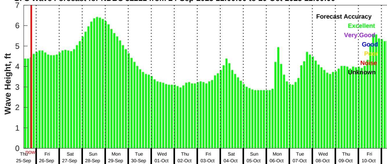
GFS Wave Forecast for NDBC 52211 from 24-Sep-2025 11:00:00 to 10-Oct-2025 11:00:00
