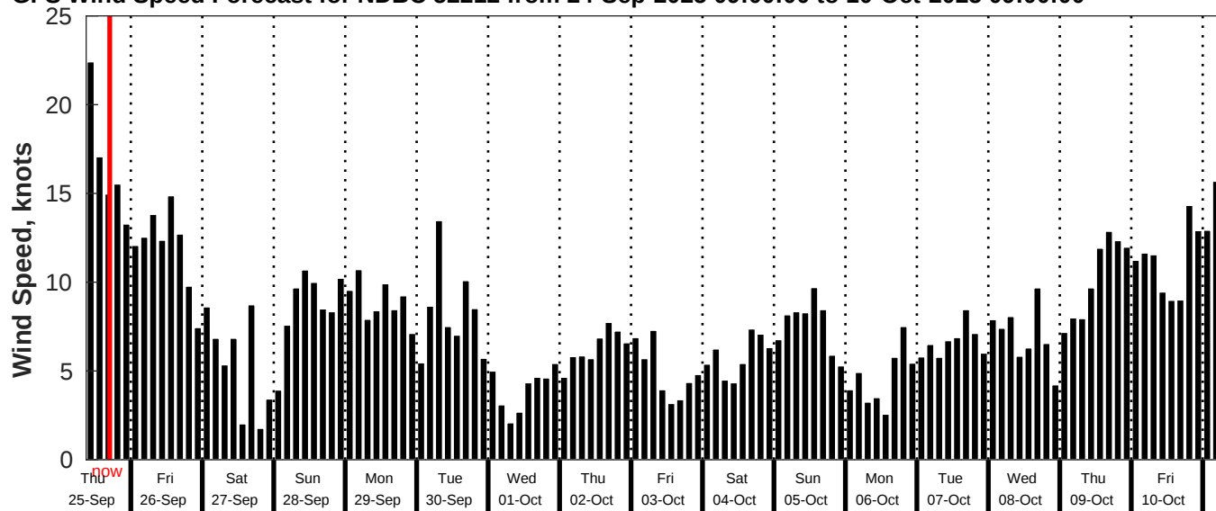
GFS Wind Speed Forecast for NDBC 52212 from 24-Sep-2025 09:00:00 to 10-Oct-2025 09:00:00
