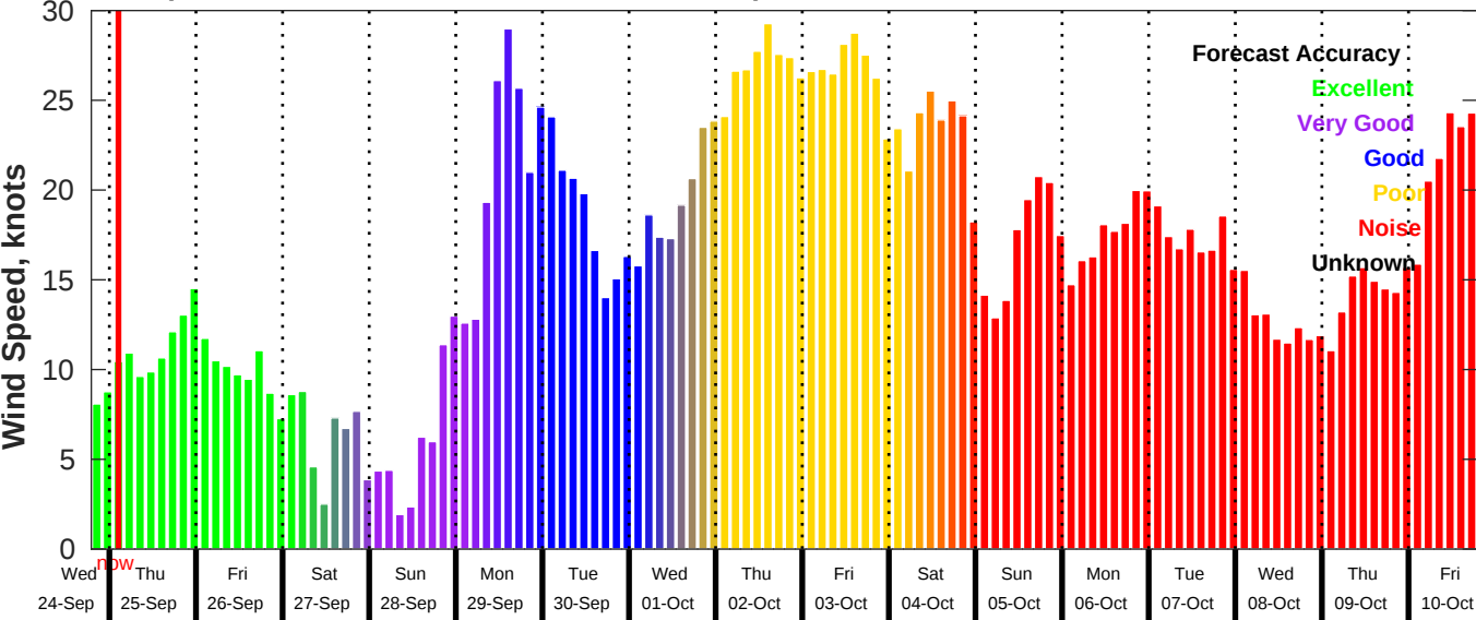
GFS Wind Speed Forecast for NDBC 41004 from 24-Sep-2025 19:00:00 to 10-Oct-2025 19:00:00
