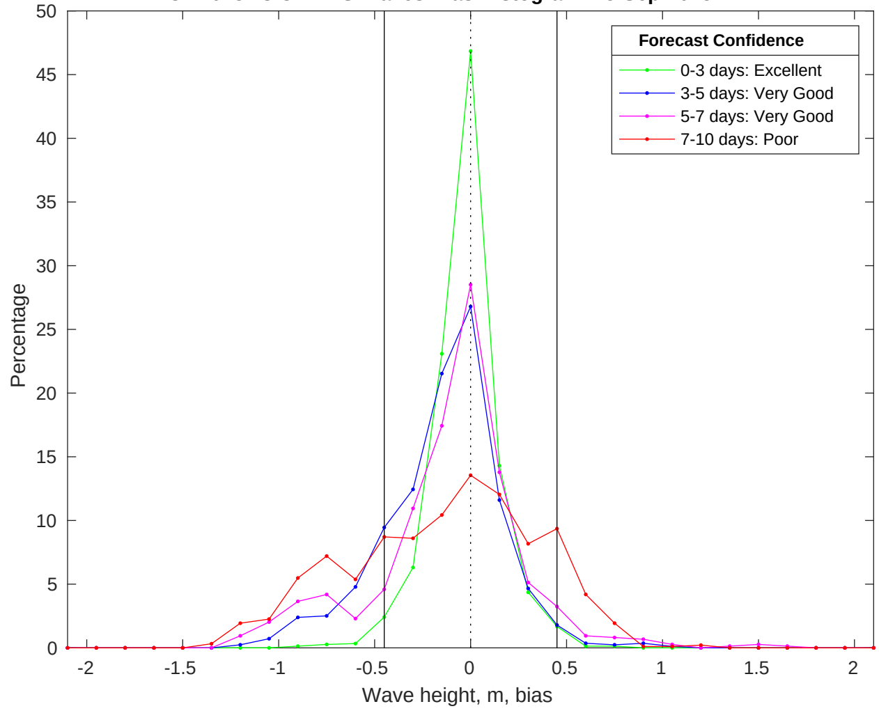
NDBC 41013 vs CMEMS Waves Bias Histogram: 25-Sep-2025
