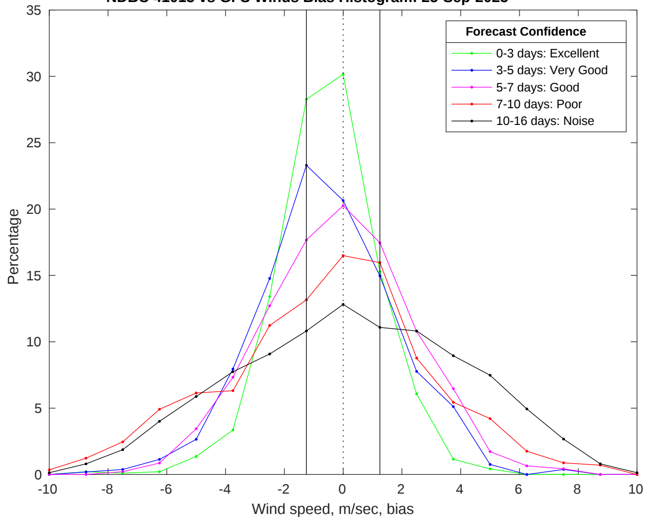
NDBC 41013 vs GFS Winds Bias Histogram: 25-Sep-2025
