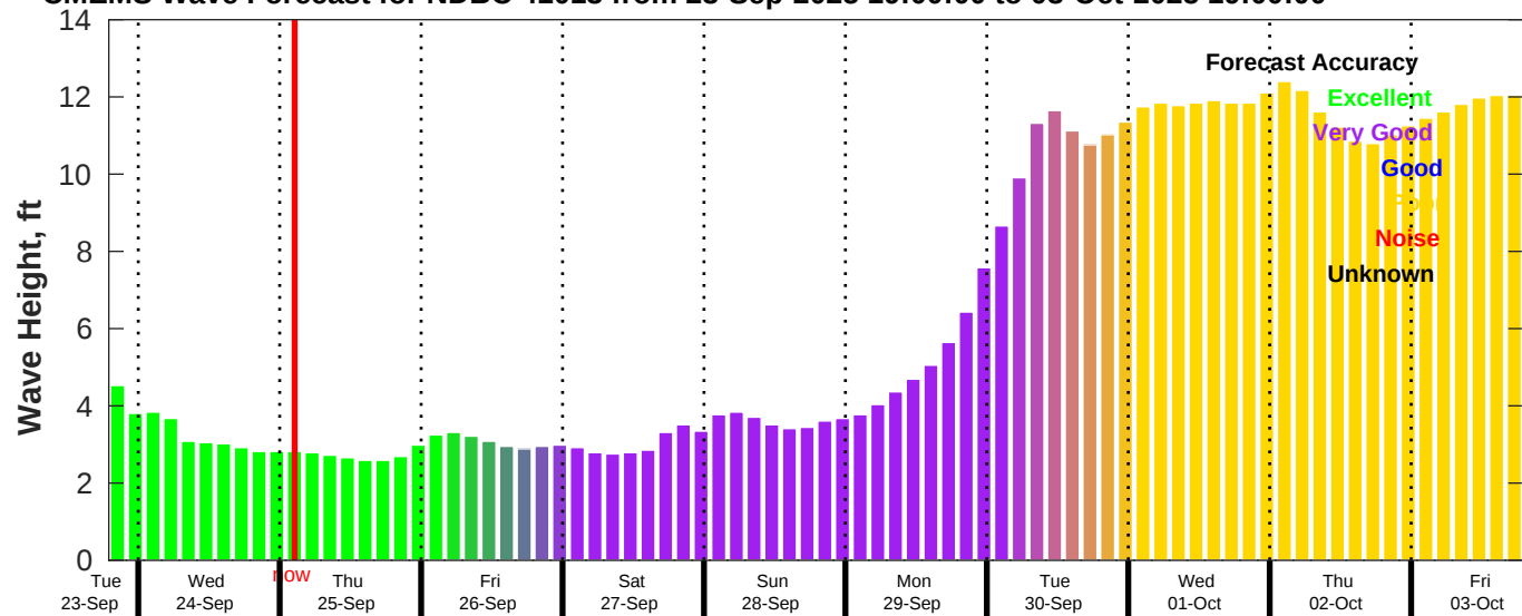
CMEMS Wave Forecast for NDBC 41013 from 23-Sep-2025 19:00:00 to 03-Oct-2025 19:00:00
