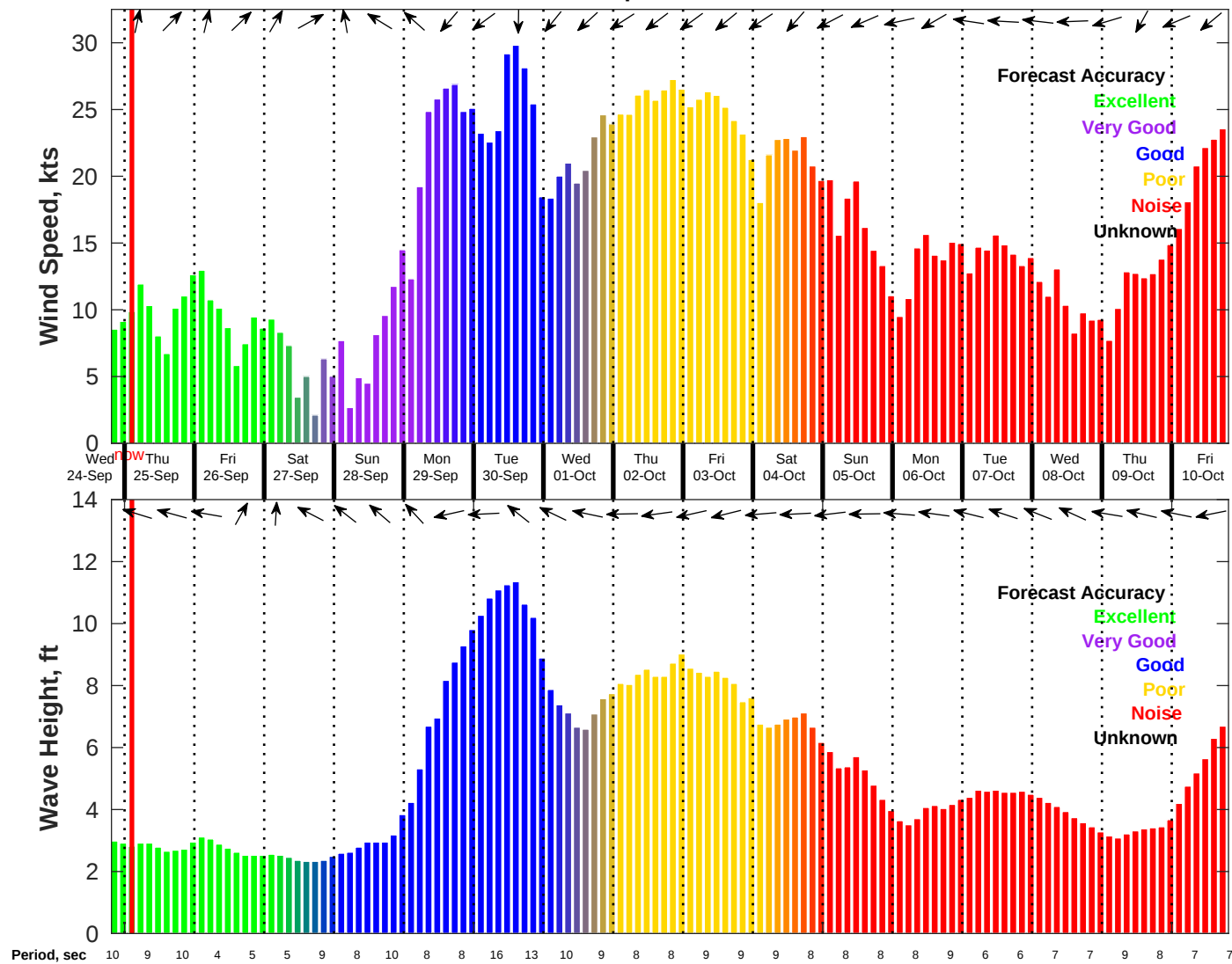
Wind & Wave Forecast for NDBC 41013 from 24-Sep-2025 19:00:00 to 10-Oct-2025 19:00:00
