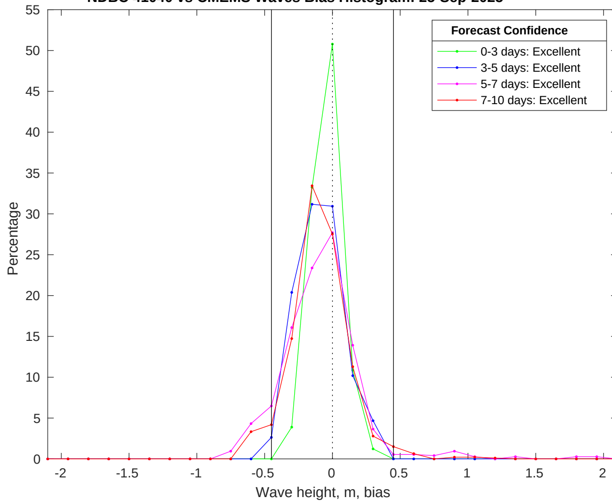
NDBC 41040 vs CMEMS Waves Bias Histogram: 25-Sep-2025
