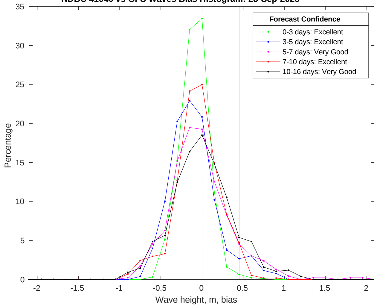
NDBC 41040 vs GFS Waves Bias Histogram: 25-Sep-2025
