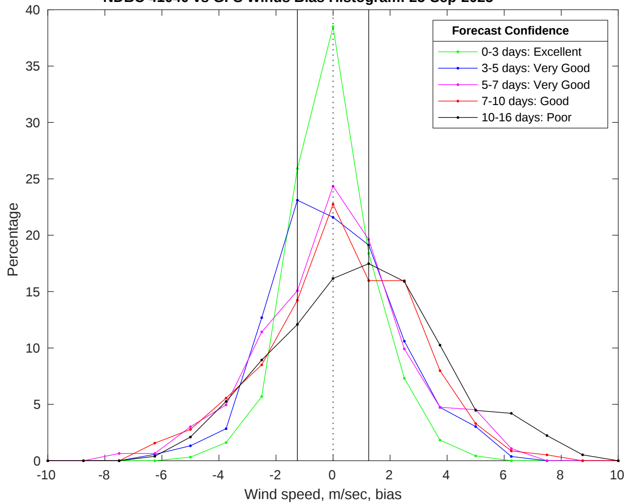
NDBC 41040 vs GFS Winds Bias Histogram: 25-Sep-2025
