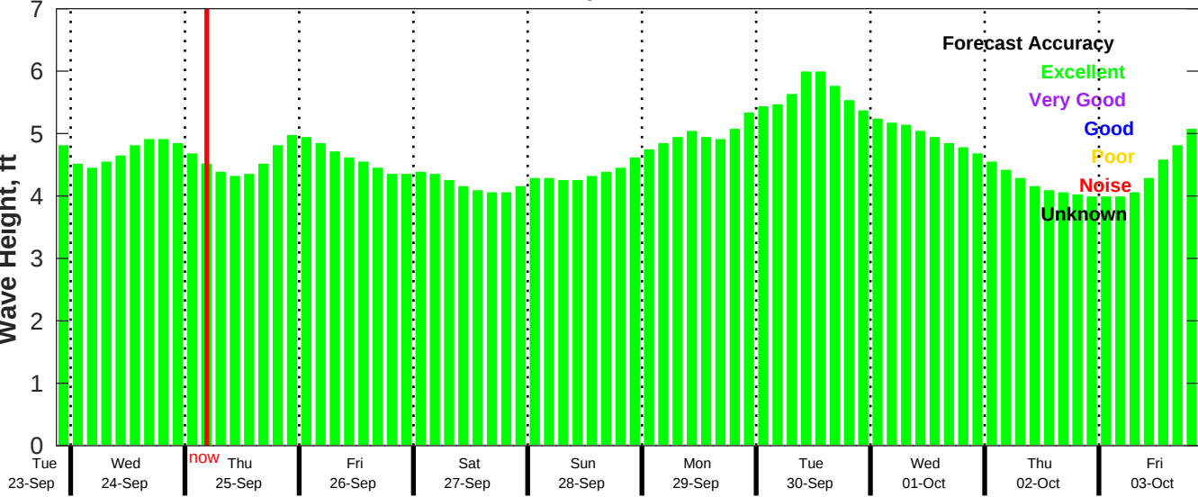
CMEMS Wave Forecast for NDBC 41040 from 23-Sep-2025 21:00:00 to 03-Oct-2025 21:00:00
