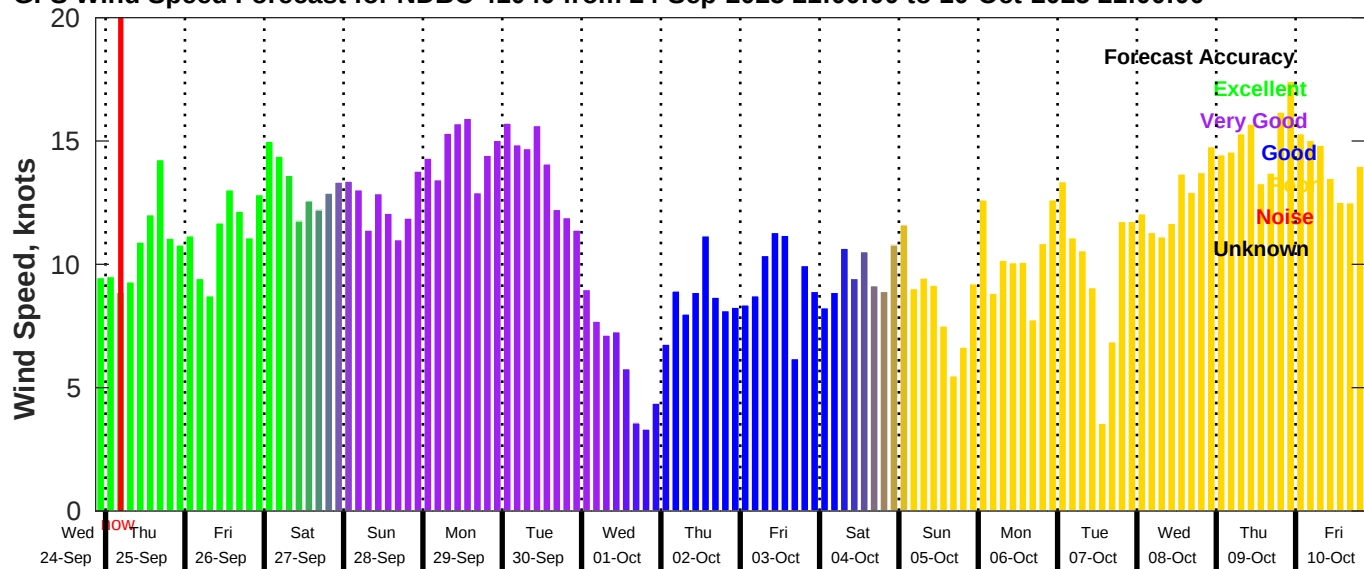
GFS Wind Speed Forecast for NDBC 41040 from 24-Sep-2025 21:00:00 to 10-Oct-2025 21:00:00
