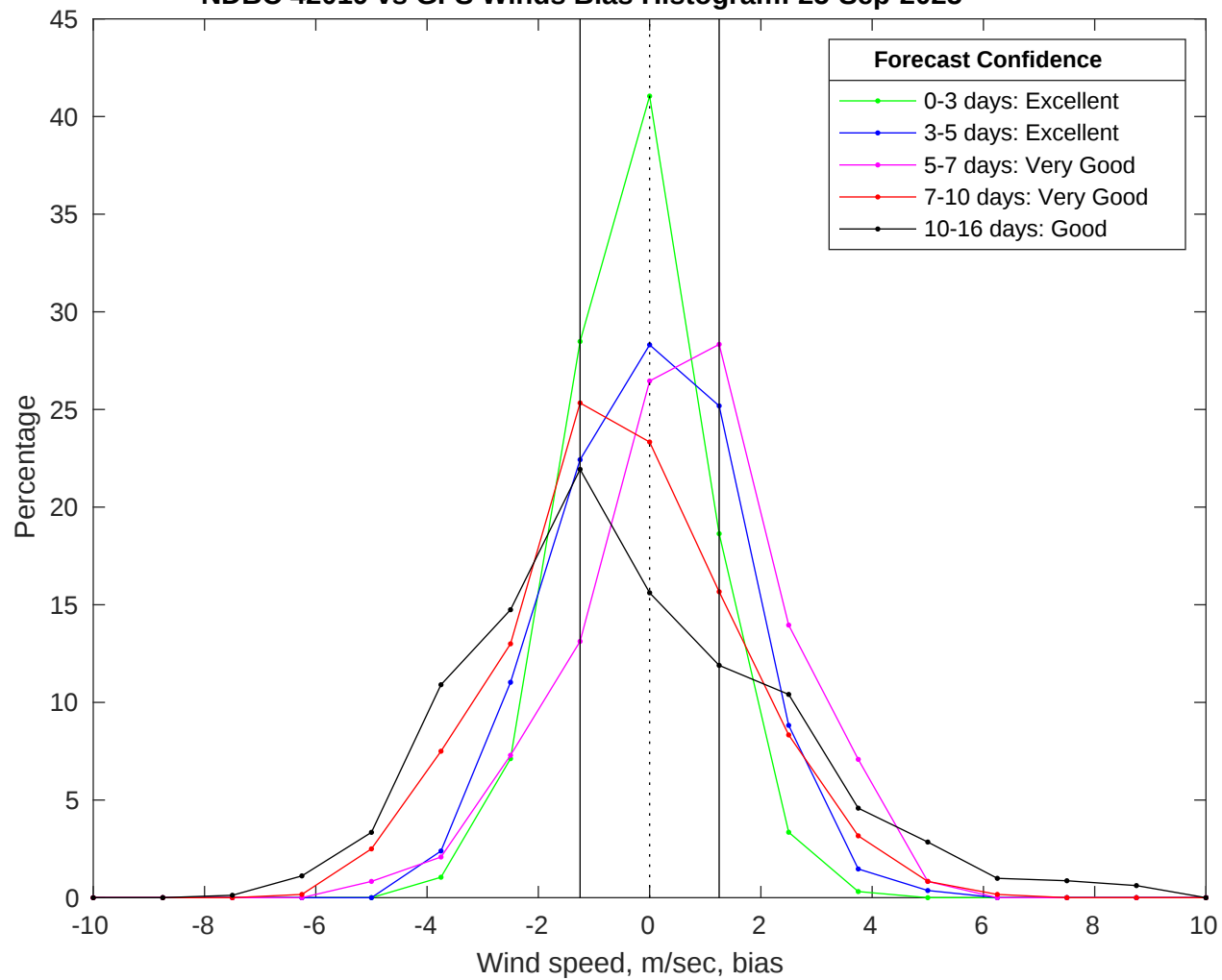
NDBC 42019 vs GFS Winds Bias Histogram: 25-Sep-2025
