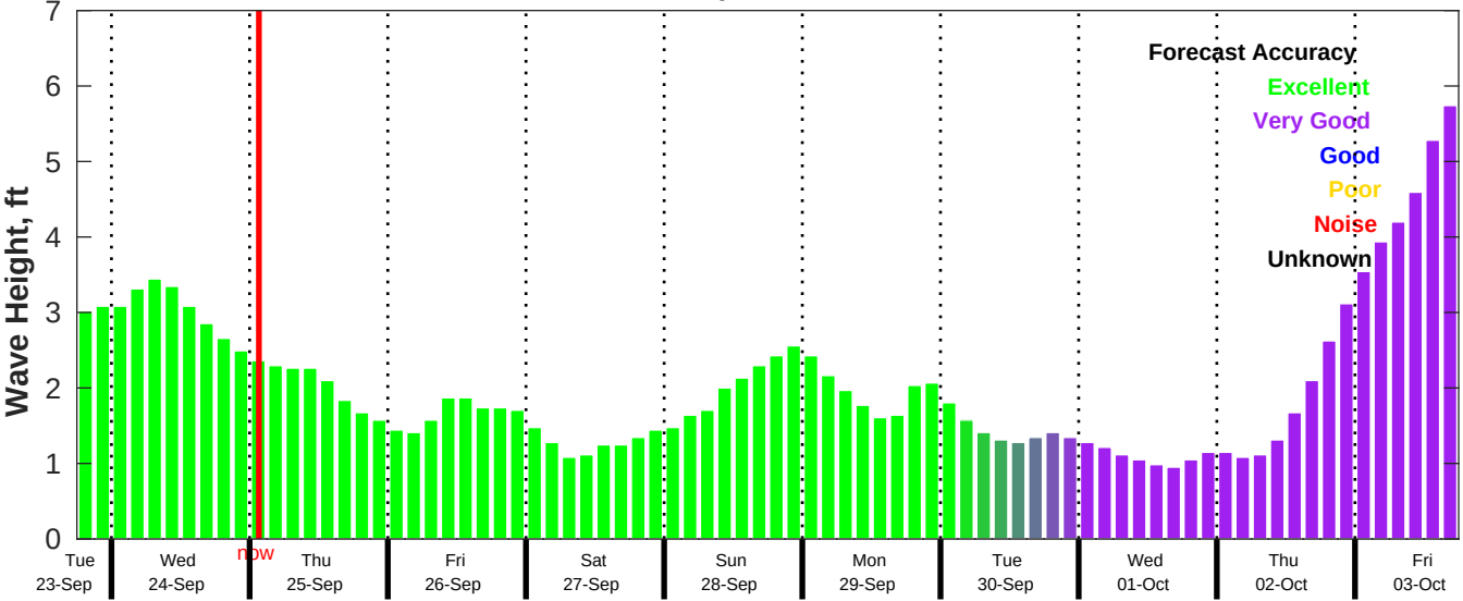
CMEMS Wave Forecast for NDBC 42019 from 23-Sep-2025 18:00:00 to 03-Oct-2025 18:00:00
