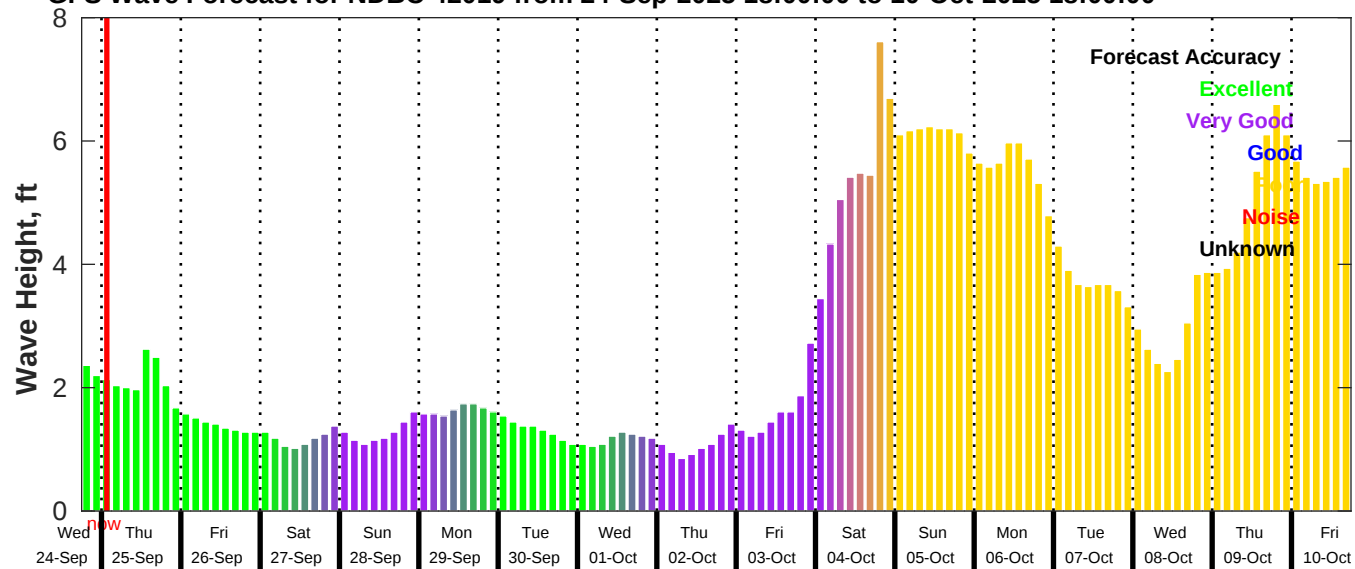
GFS Wave Forecast for NDBC 42019 from 24-Sep-2025 18:00:00 to 10-Oct-2025 18:00:00
