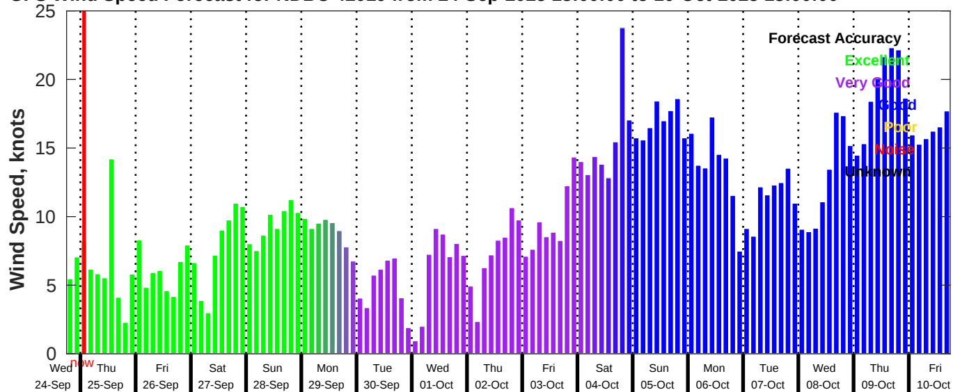
GFS Wind Speed Forecast for NDBC 42019 from 24-Sep-2025 18:00:00 to 10-Oct-2025 18:00:00
