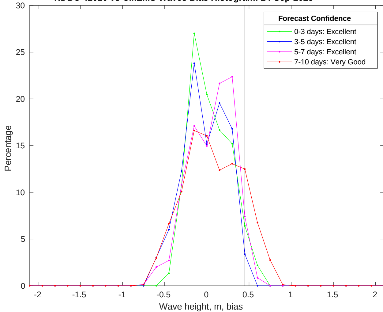
NDBC 42020 vs CMEMS Waves Bias Histogram: 24-Sep-2025
