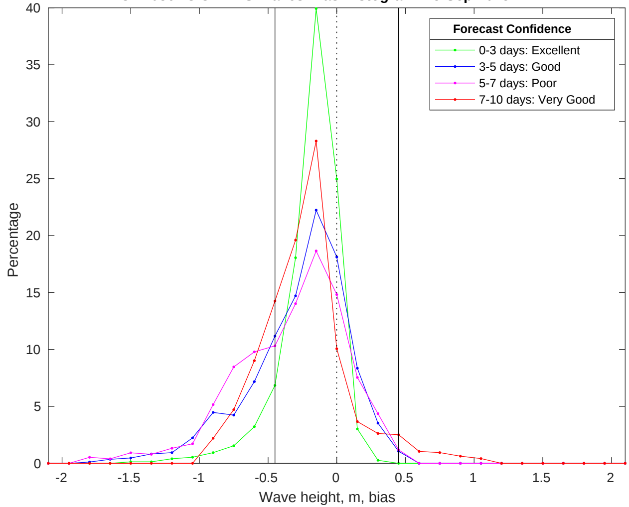
NDBC 42036 vs CMEMS Waves Bias Histogram: 25-Sep-2025
