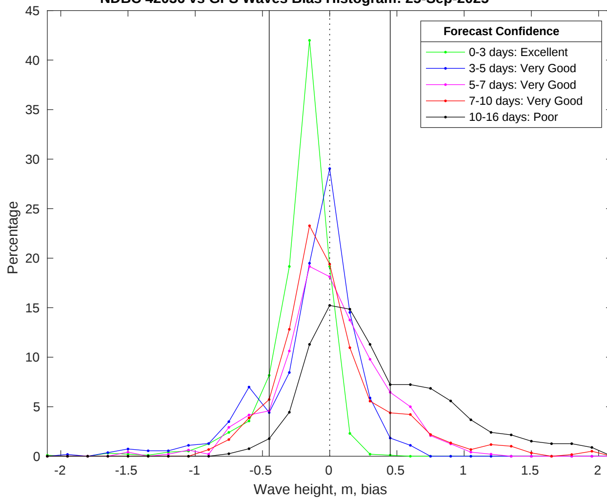
NDBC 42036 vs GFS Waves Bias Histogram: 25-Sep-2025
