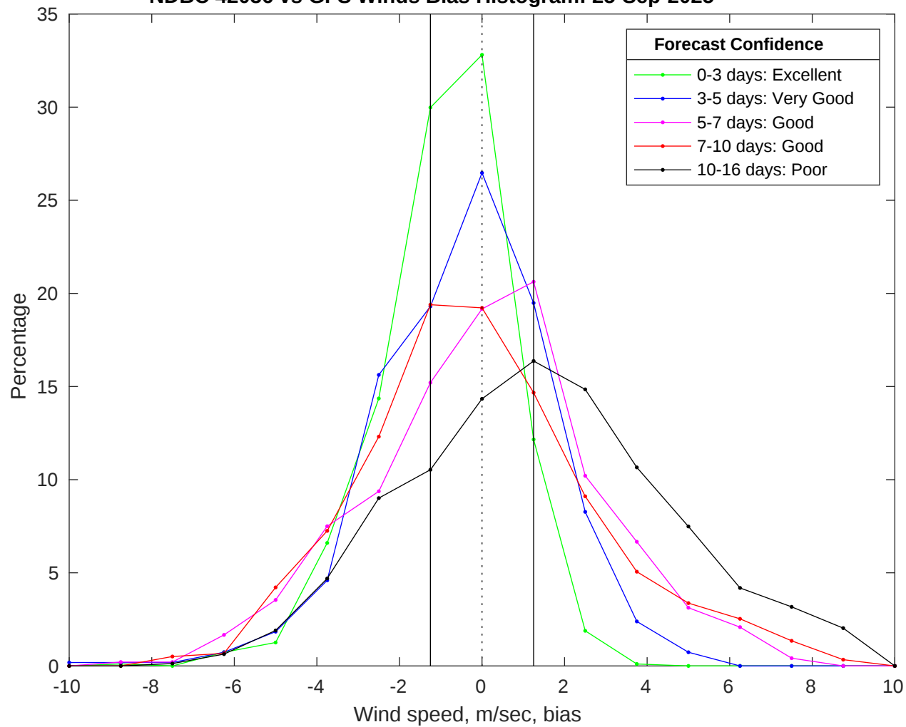
NDBC 42036 vs GFS Winds Bias Histogram: 25-Sep-2025
