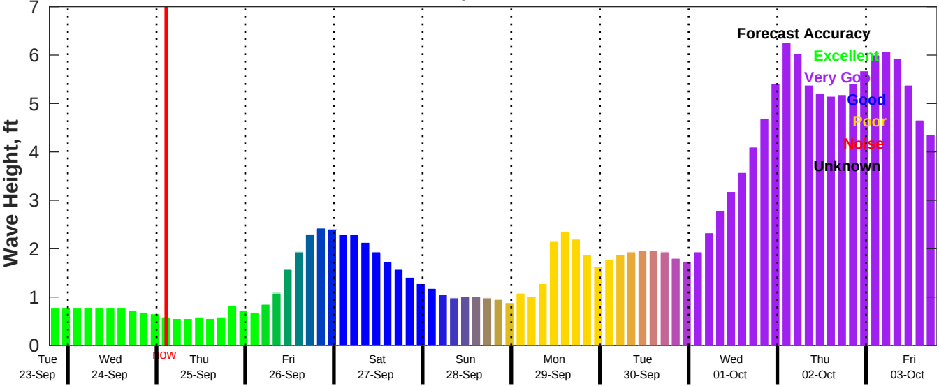
CMEMS Wave Forecast for NDBC 42036 from 23-Sep-2025 19:00:00 to 03-Oct-2025 19:00:00
