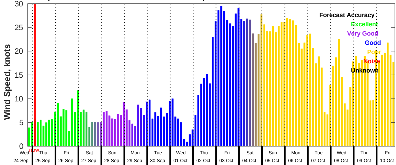
GFS Wind Speed Forecast for NDBC 42036 from 24-Sep-2025 19:00:00 to 10-Oct-2025 19:00:00
