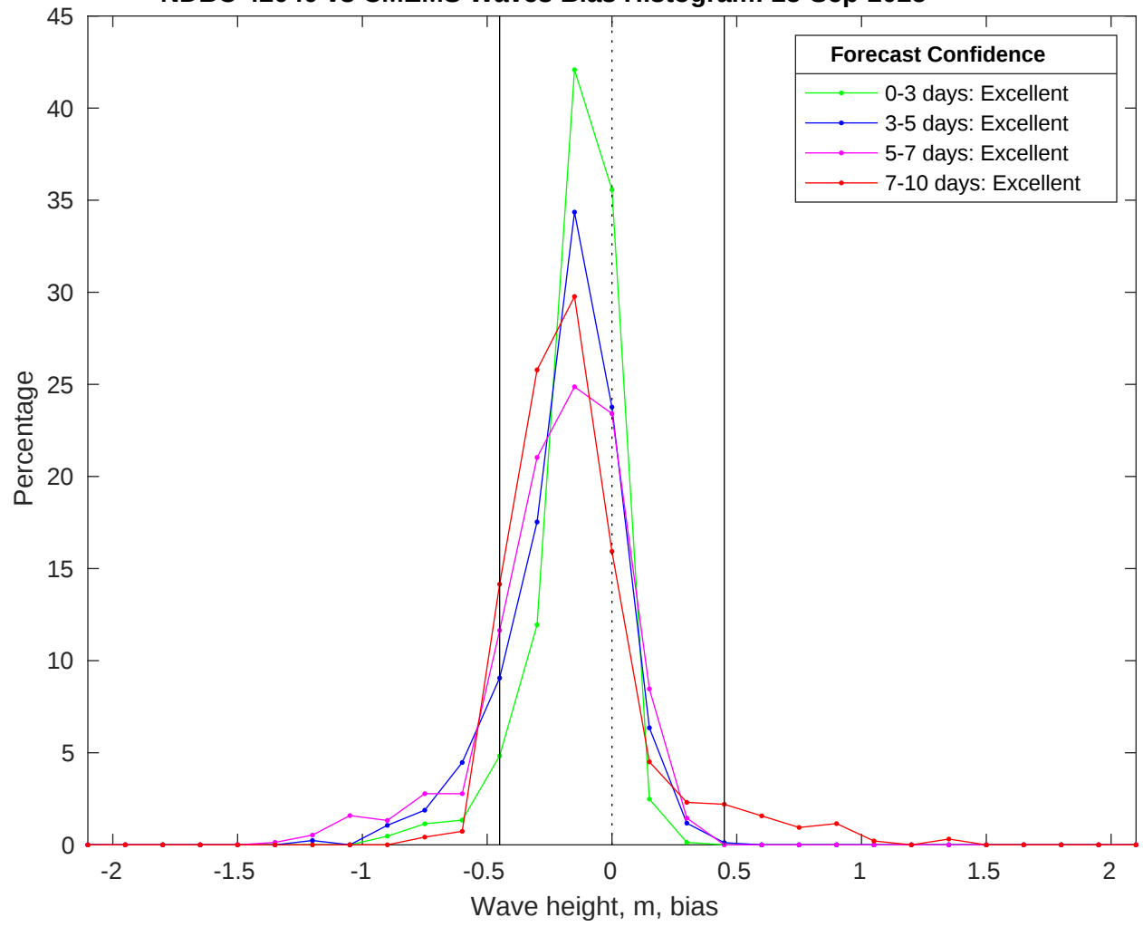
NDBC 42040 vs CMEMS Waves Bias Histogram: 25-Sep-2025
