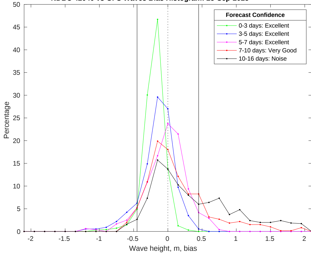
NDBC 42040 vs GFS Waves Bias Histogram: 25-Sep-2025
