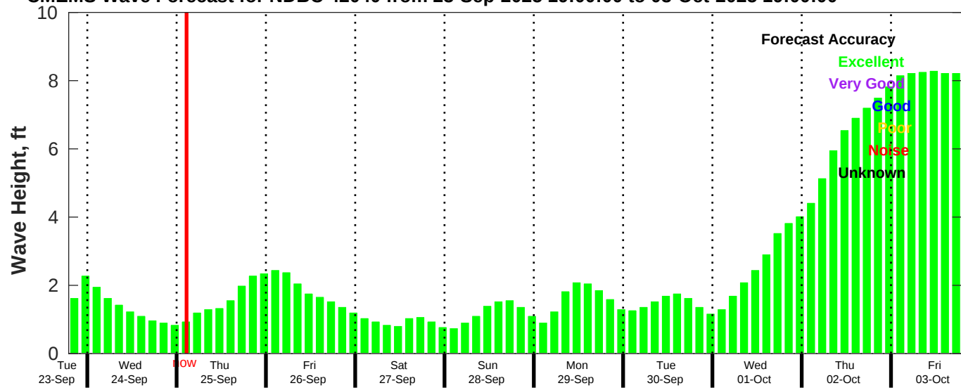
CMEMS Wave Forecast for NDBC 42040 from 23-Sep-2025 19:00:00 to 03-Oct-2025 19:00:00
