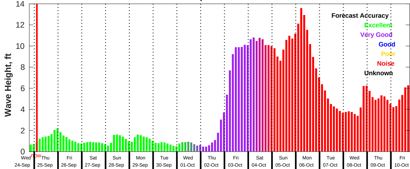
GFS Wave Forecast for NDBC 42040 from 24-Sep-2025 19:00:00 to 10-Oct-2025 19:00:00
