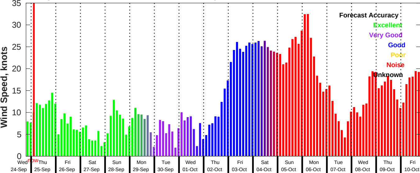
GFS Wind Speed Forecast for NDBC 42040 from 24-Sep-2025 19:00:00 to 10-Oct-2025 19:00:00
